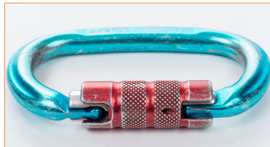
Connector with sleeve which doesn't automatically return to the locked position. ⚠ Lubricate the sleeve as indicated in the user instructions. If the problem is not completely resolved, scrap the device.
