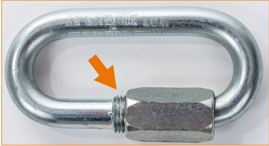
Quicklink with the screw-up sleeve screwed beyond allowed limit.
