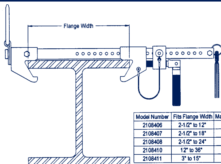
Figure 2 - Beam Flange Application Sizes
