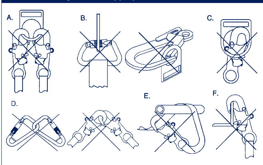
Figure 5 - Inappropriate Connections
