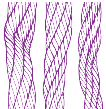
Kinked wire ropes which have been used. Kinks are pulled tight and caused distortion and failure.
