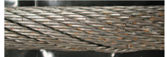
Crown wire breaks on a Python® Lift non-rotating wire rope
